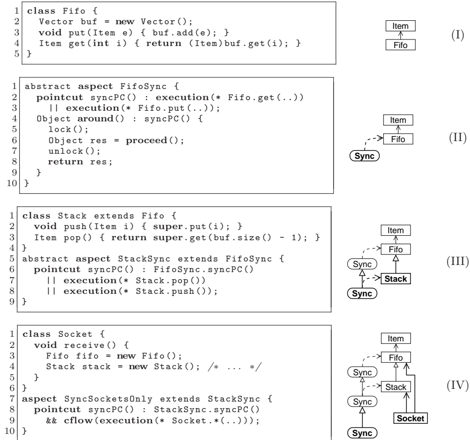
Fig. 1. A SWR example using aspects (AspectJ code).
