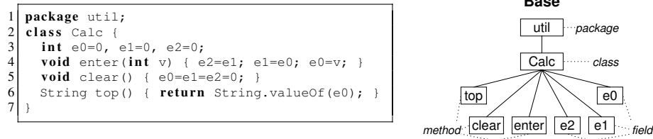
Fig. 1. Implementation and FST of the feature Base
