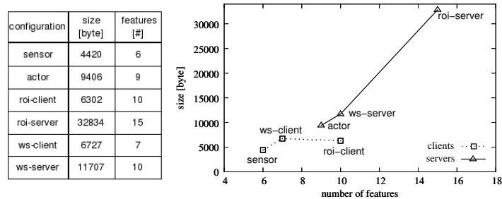
Fig. 10. Memory footprint and number of features of three configurations
