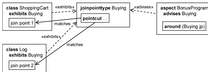
Fig. 4. Classes ShoppingCart and Log both depend on the join point type Buying , as does aspect BonusProgram (dashed arrows). The pointcut defined in Buying matches join points in the classes, and is used to trigger the advice in BonusProgram . Note how this corresponds to Figure 3(c).
