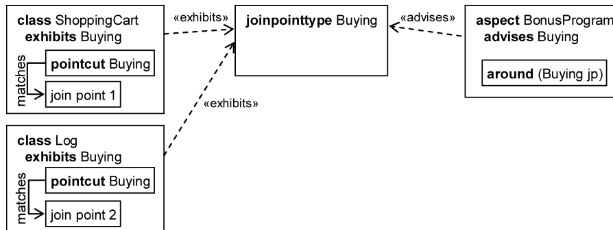
Fig. 5. Polymorphic pointcuts removing the dependency of join point types on exhibiting classes. The decoupling achieved is thus that of Figure 3(d). Note how polymorphic pointcuts resemble interface implementation in JAVA ; here, however, (implicit) method invocations, not methods, are implemented.
