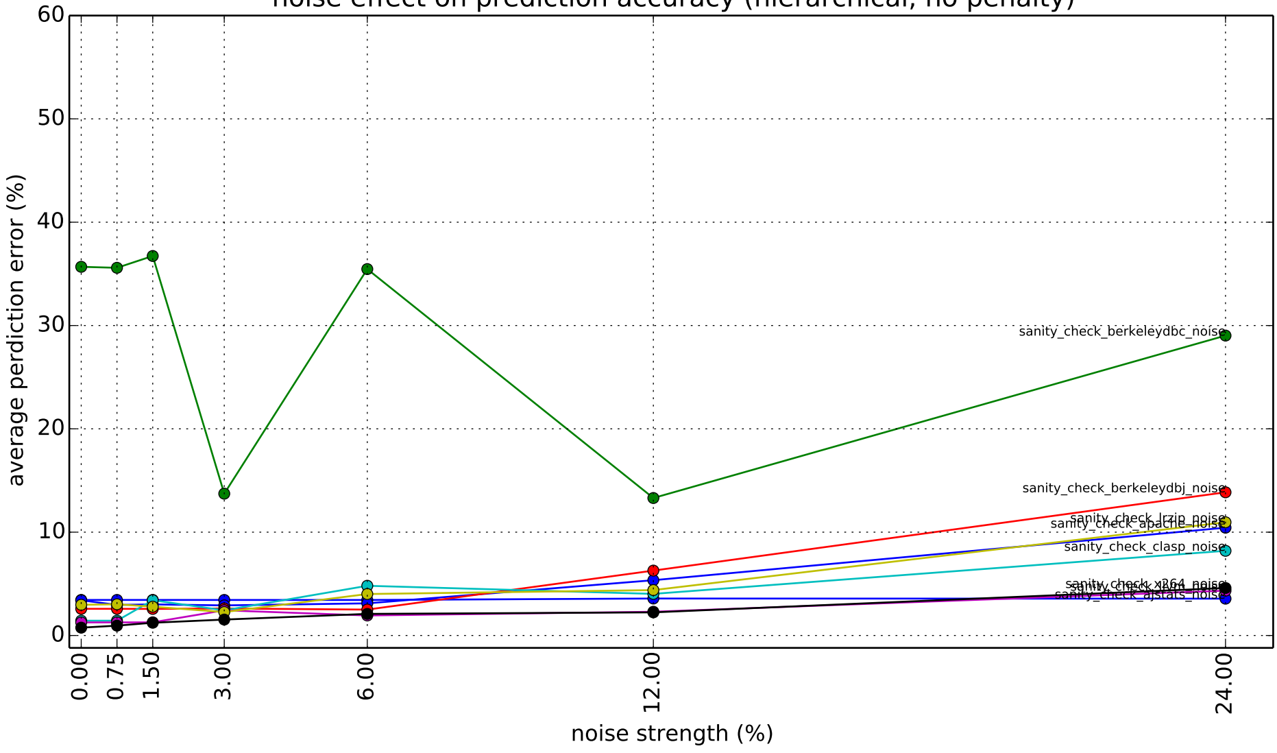
noise effect on prediction accuracy (hierarchical, with penalty)
